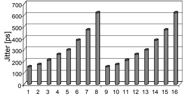
Fig. 9. Timing error accumulation for eight-stage delay chain when simulation was done at 20MHz
