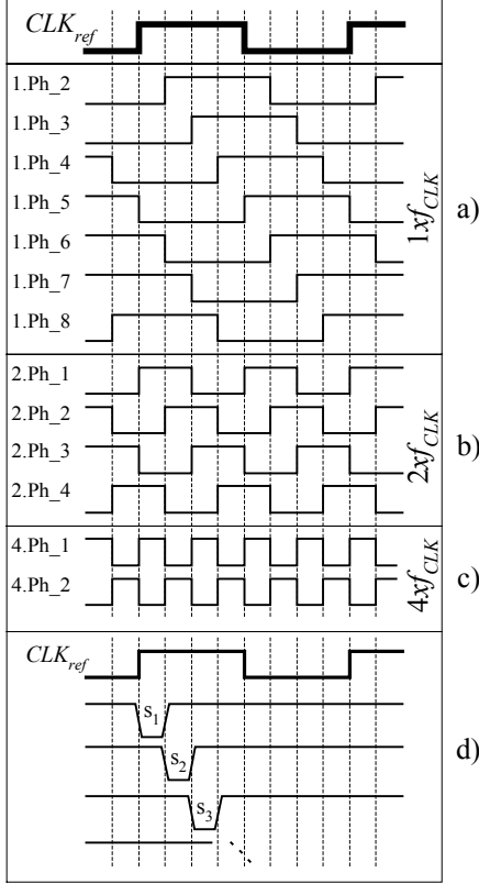
Fig. 4. Poly-phase and referent clock multiplier
