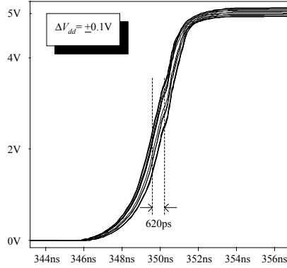
Fig. 7. Simulated tracking jitter with \pm 100\text{mV} supply noise
