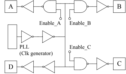
Fig. 2. Clock-gating and clock networks
