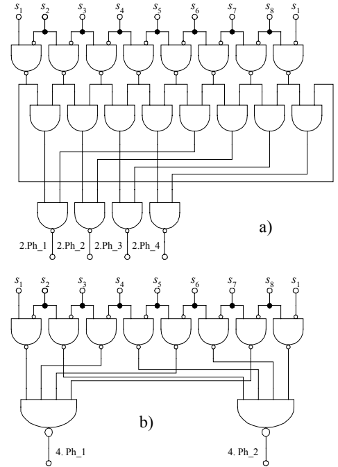
Fig. 6 a) Four phases double f_{CLK} frequency multiplier b) Two phases quadruple f_{CLK} frequency multiplier
