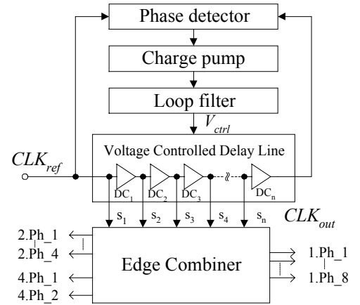
Fig. 3. Multi-frequency and multi-phase DLL frequency synthesizer
