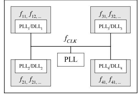
Fig. 1. Clock distribution architecture using PLL or DLL
