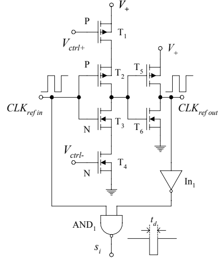
Fig. 5. Voltage controlled delay cell with pulse generator
