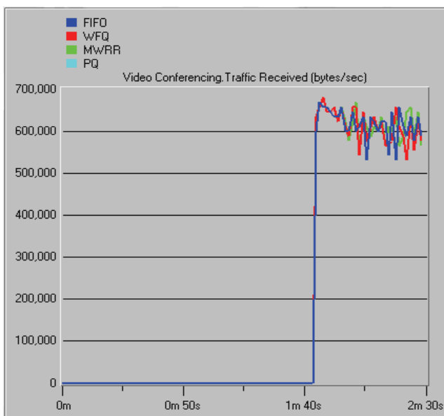
Fig. 4. Video-conferencing traffic received (bytes/sec)
