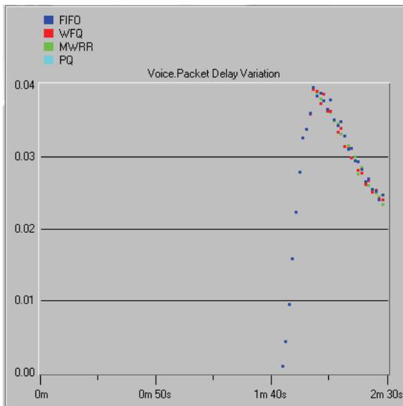
Fig. 7. Voice packet delay variation (sec)
