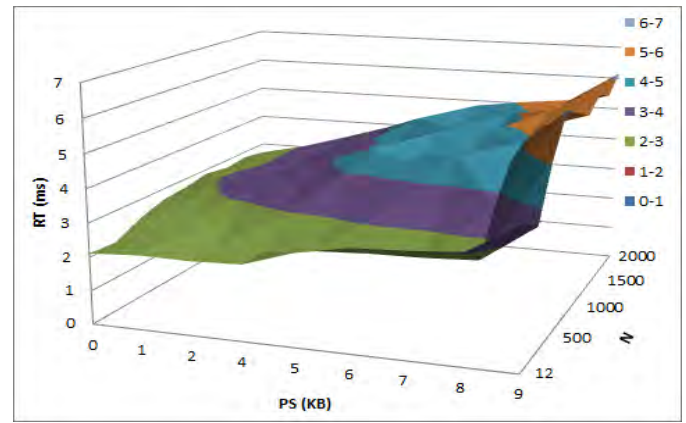
Figure 4. Concat WS response time in virtual environment
