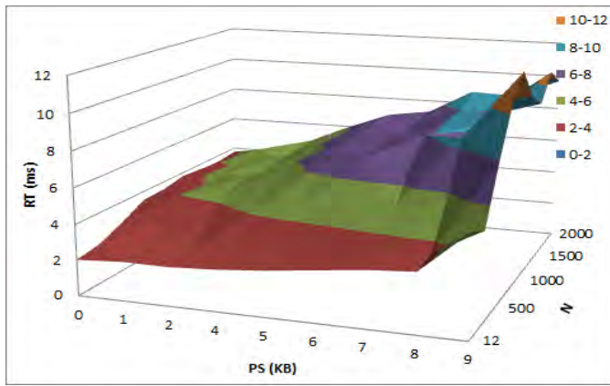
Figure 2. Concat WS response time on bare metal machine
