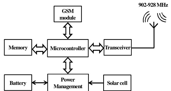
Fig 3. Block diagram of retranslating base station.
