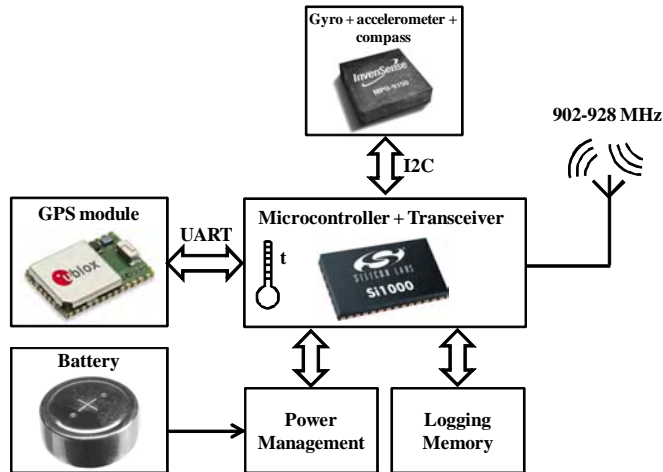
Fig 2. Block diagram of the tracking device (tag).
