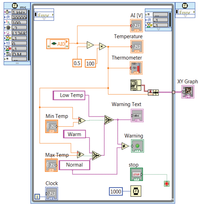
Fig.5. Block diagram of the measuring system
