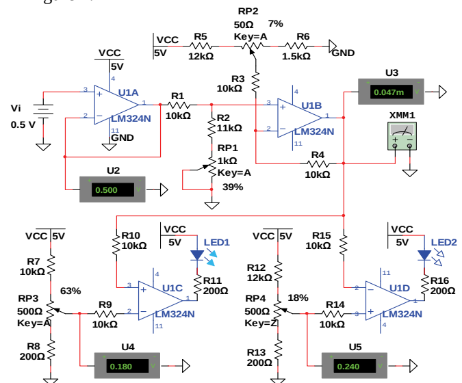
Fig.4. Circuit design of temperature transducer
