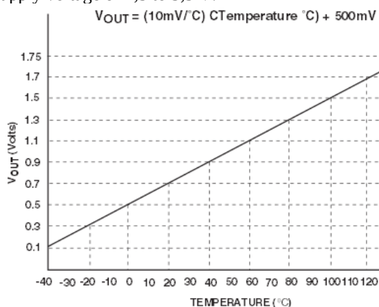
Fig.3. Dependence U_{out} = \varphi(T) for TC1047A
