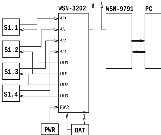
S1.1 ÷ S1.4 – sensors (temperature, humidity, noise, light); PWR – battery power supply for the sensors; WSN-3202 – node; BAT – battery power supply for the node; WSN-9791 – gateway; Fig.2. Functional scheme of the system collecting data
