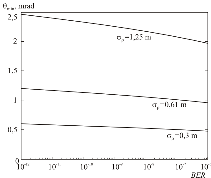
Fig.2. Dependence of minimum divergence angle on Bit-Error Rate for various values of \sigma_p and Z=3000 m
