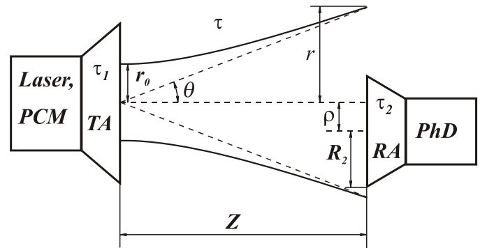
Fig. 1. FSO system
