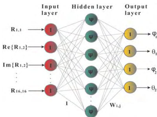
Fig. 2. RBF neural model for 2D DOA estimation of coherent sources
