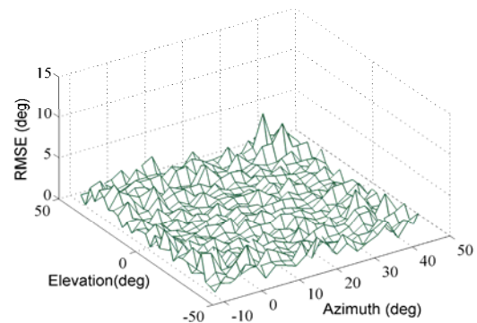
Fig. 4. RMSE of the 2D DOA estimates for the second coherent source (mutual distance between sources is 35^\circ )
