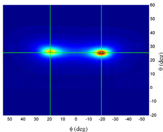
Fig. 7. MUSIC with SSP spectrum for two coherent sources positioned at (-21^\circ, 26^\circ) and (21^\circ, 26^\circ)
