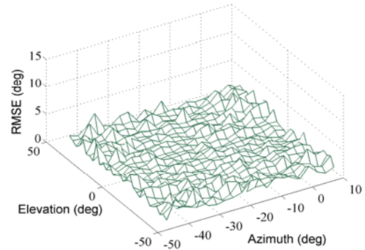
Fig. 3. RMSE of the 2D DOA estimates for the first coherent source (mutual distance between sources is 35^\circ )
