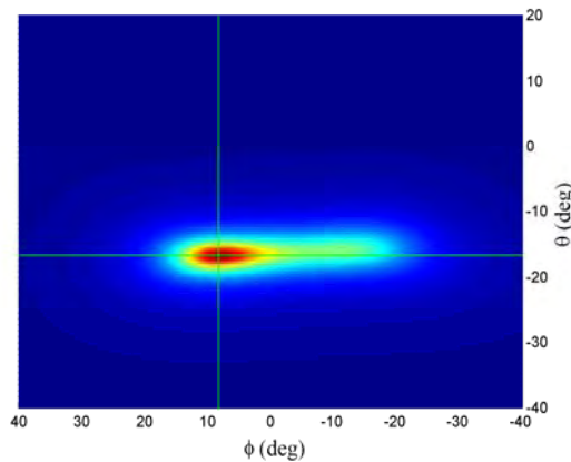
Fig. 6. MUSIC with SSP spectrum for two coherent sources positioned at (-14^\circ, -17^\circ) and (14^\circ, -17^\circ)
