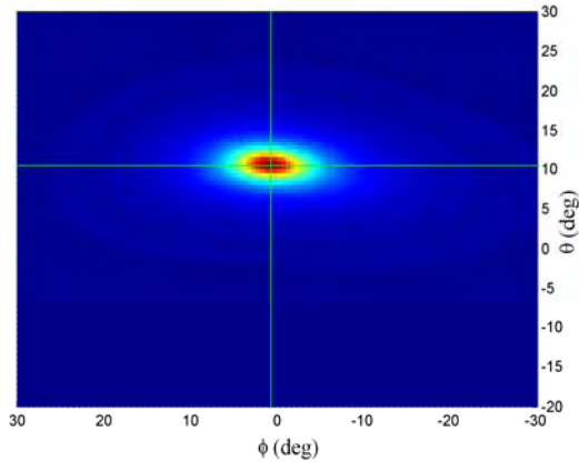
Fig. 5. MUSIC with SSP spectrum for two coherent sources positioned at (-10^\circ, 10^\circ) and (-10^\circ, 10^\circ)
