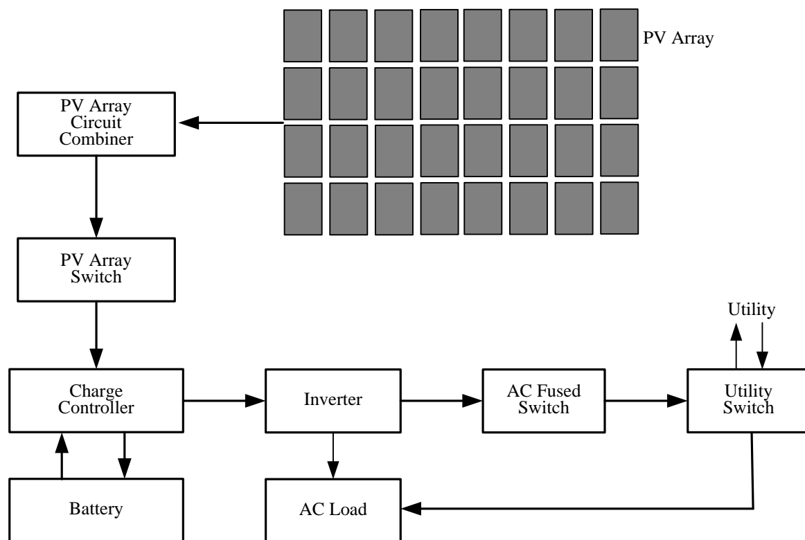
Fig. 2. Principle of operation of the designed solar PV system
