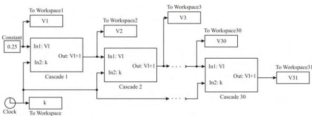
Fig. 8. Bondsime model of system given in Fig. 4
