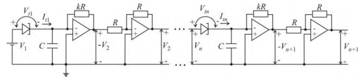
Fig. 4. System of 30 cascade connected electrical circuits in the case of the quasi steady state
