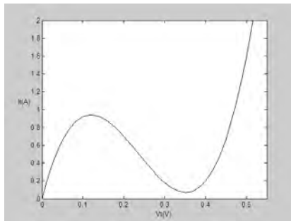
Fig. 1. Current – voltage characteristic of tunnel diode
