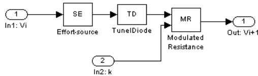
Fig. 6. Bondsime model of one cascade
