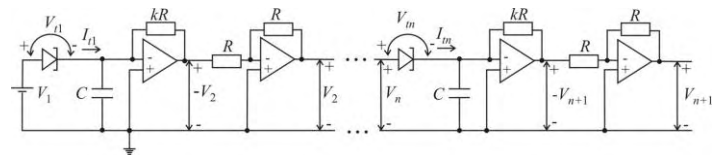
Fig. 3. System of 30 cascade connected electrical circuits
