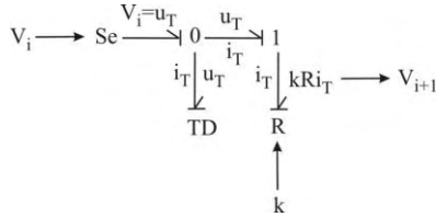
Fig. 5. Bond graph model of one cascade
