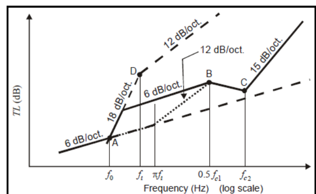
Fig. 1. A design chart for estimating the transmission loss of a double panel wall, based on Sharp’s analysis
