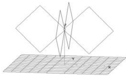
FIG. 8 – DOUBLE BIQUAD ANTENNA WITH REFLECTOR– PRINCIPLED SCHEME
