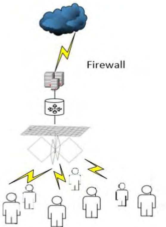
Figure 9 – An example of practice application of 2biQUAD antenna with reflector in Wi-Fi frequency band
