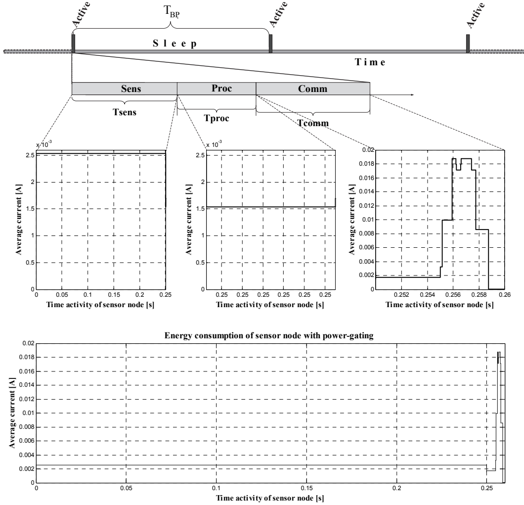
Fig. 3. Activity profile of the sensor node
