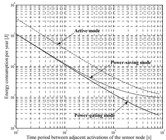
Fig. 2. Total energy consumption for three cases
