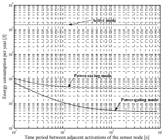
Fig. 4. Total energy consumption in real conditions
