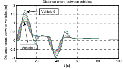
Fig. 7. Distance errors between vehicles
