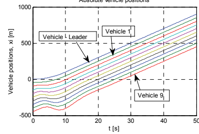
Fig. 8. Positions of the vehicles
