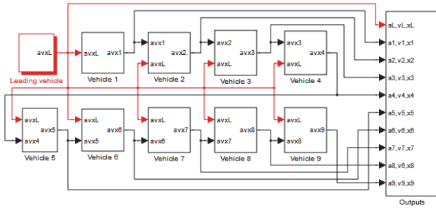
Fig. 5. Matlab/Simulink model of the platoon of 10 vehicles
