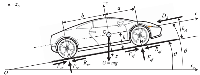
Fig. 1. Forces acting on a vehicle
