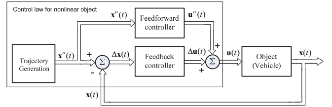
Fig. 2. Concept of feed-forward and feedback control system of nonlinear object
