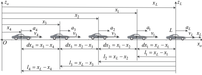
Fig. 4. Configuration of platoon with 5 vehicles
