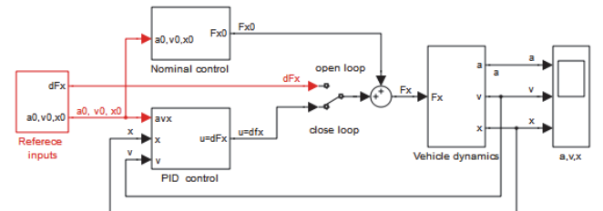
Fig. 3. Simulink diagram for the vehicle control
