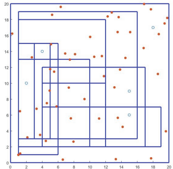
Fig. 1. Indoor wireless network environment layout based on the RIEG wall layout method
