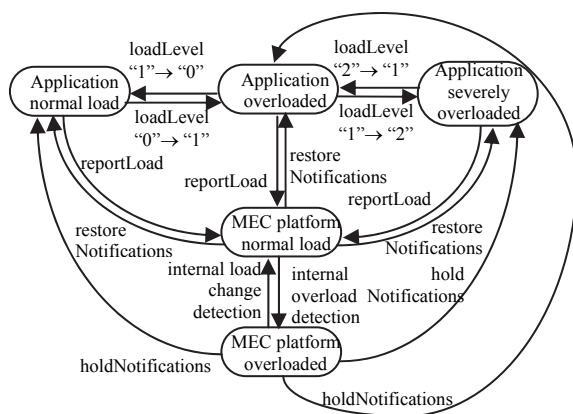
Fig. 4. Application and MEC platform load level states
