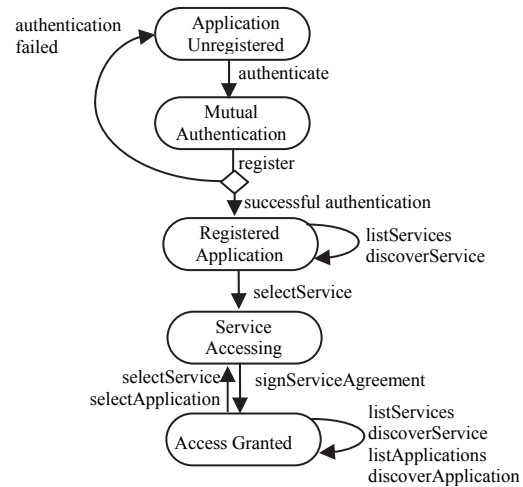
Fig. 3. Registration and access to MEC services
