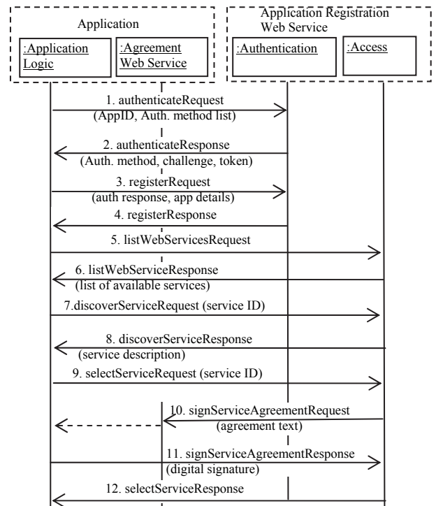
Fig. 1. Application authentication and MEC service discovery, selection and signing of service agreement
