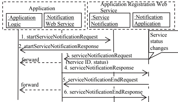
Fig. 2. Triggered notifications about changes in MEC service availability status
