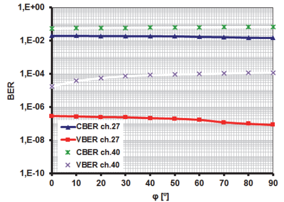
Fig. 4. BER = func(\varphi) – Rayleigh channel (monopole)
