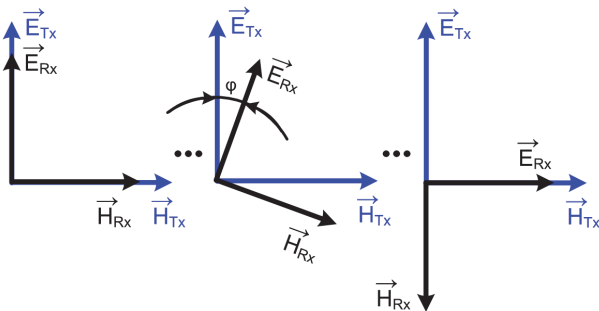
Fig. 2. Change in polarizations between Tx and Rx antennas
