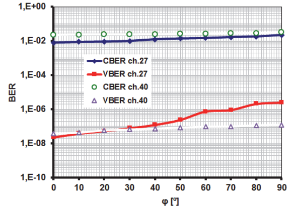
Fig. 3. BER = func(\varphi) – Ricean channel (LP-21)
