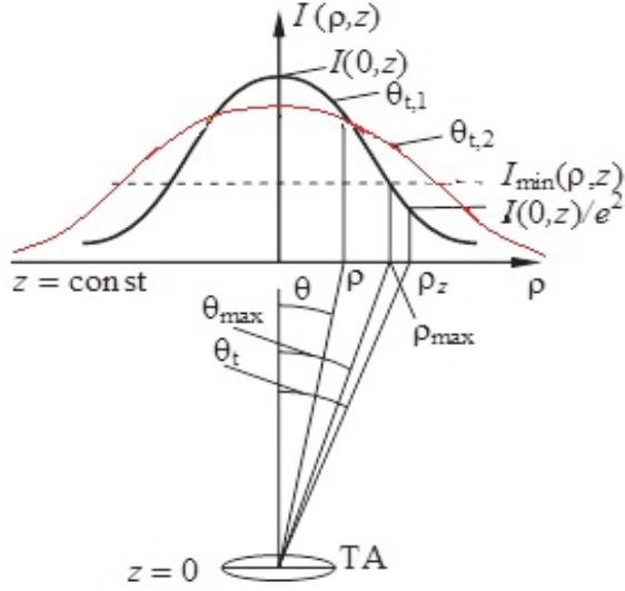
Fig. 2. Radial distribution of the intensity in a plane z = \text{const} for two values of the divergence of the optical radiation \theta_t
