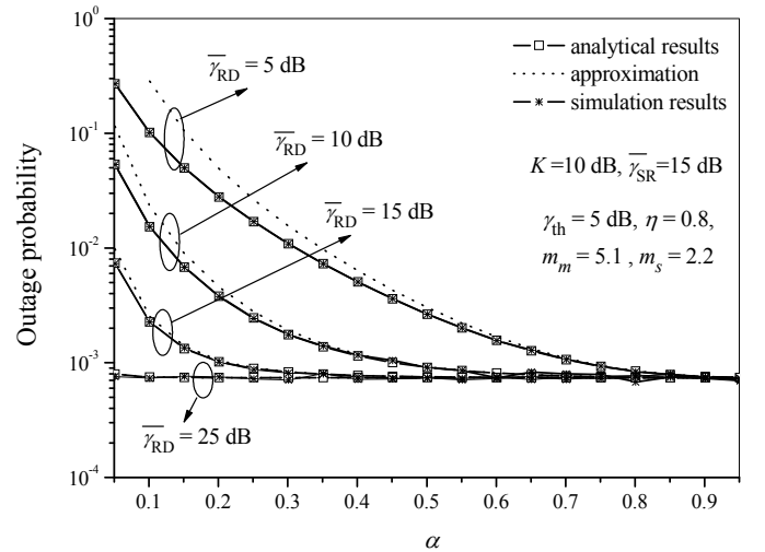
Fig. 2. Outage probability versus energy harvesting ratio for various values of average SNR of second hop
