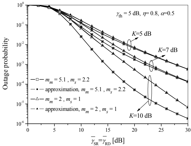
Fig. 3. Outage probability versus average SNR for various fading and shadowing conditions
