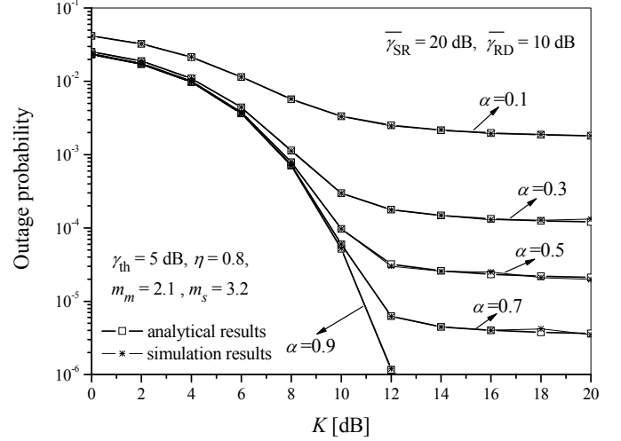
Fig. 1. Outage probability versus Rician K factor for various values of energy harvesting ratio
