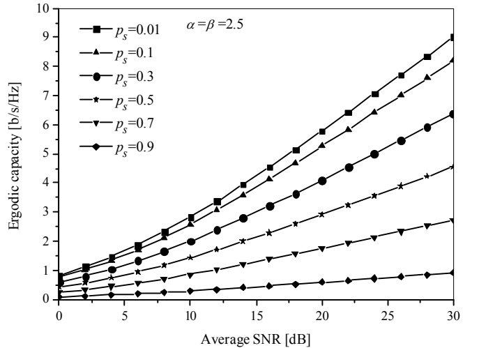
Fig. 2. Ergodic capacity versus the average SNR for different values of probability of blockage
