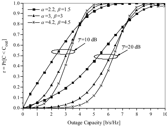
Fig. 3. Probability of channel capacity being less than the outage capacity for different fading/shadowing conditions
