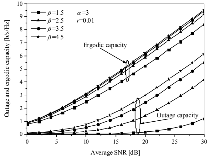
Fig. 1. Ergodic and outage capacity versus the average SNR for different values of fading severity parameter
