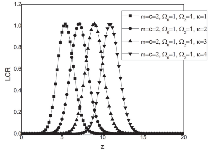
Fig. 2. Level crossing rate (LCR) depending on the envelope z , when m=c=2 , \Omega_0=1 and different values of \kappa
