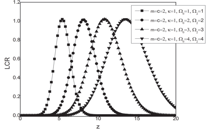
Fig. 1. Level crossing rate (LCR) depending on the envelope z , when m=c=2 , \kappa=1 and different values of \Omega_0 and \Omega_2
