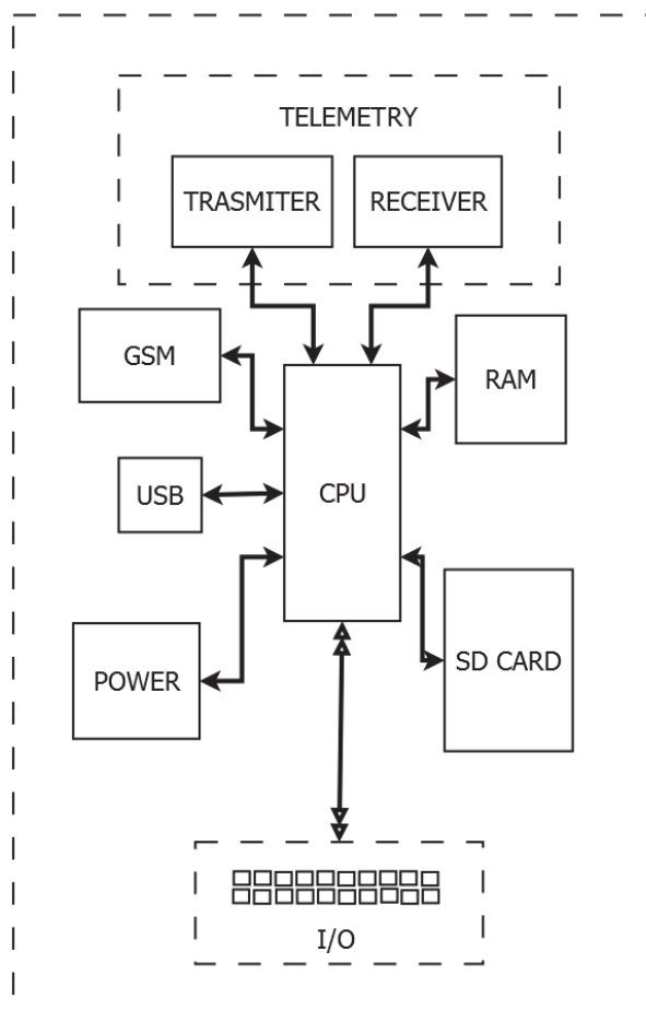
Fig. 1. Architecture of a multi-purpose development platform
