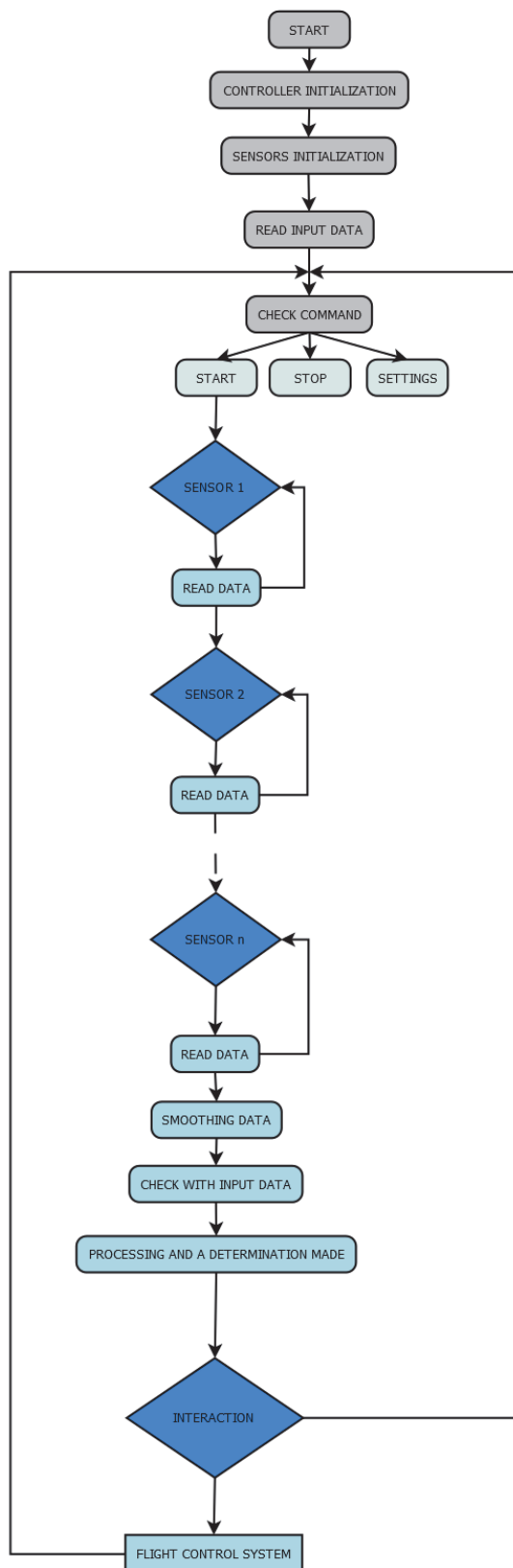
Fig. 3. Algorithm for operation of the system for flight control and technical condition for collecting and processing data from sensors onboard the UAS
