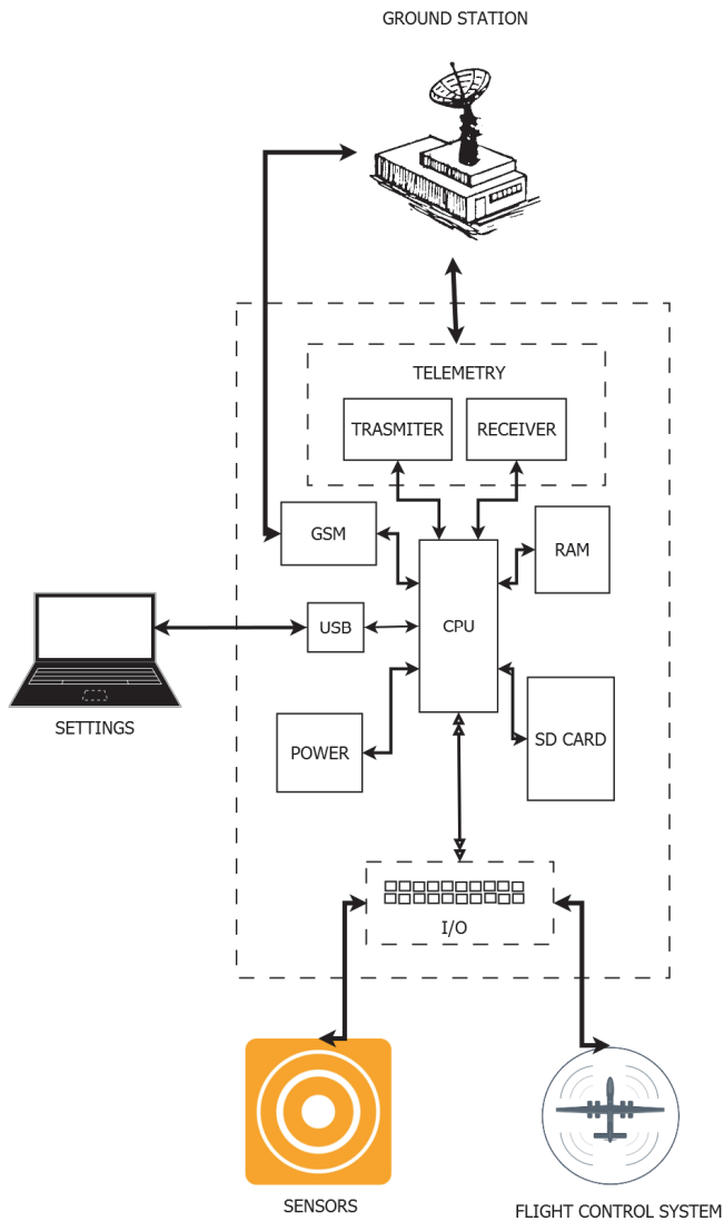
Fig. 2. Multi-purpose development platform
