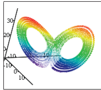
Fig.4. Chaotic mode at K = 0.2
