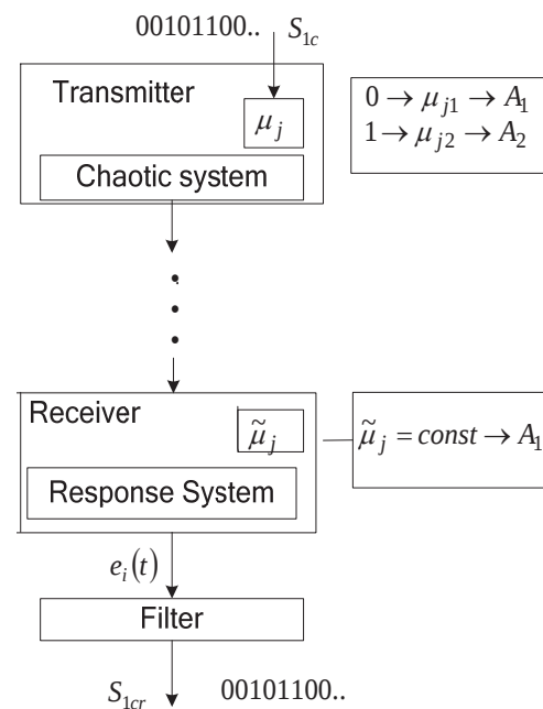
Fig. 1. A principle block diagram of the CS with CSK
