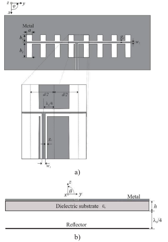
Fig. 3. CPW-fed asymmetrical slot array: a) Top view b) Side view.
