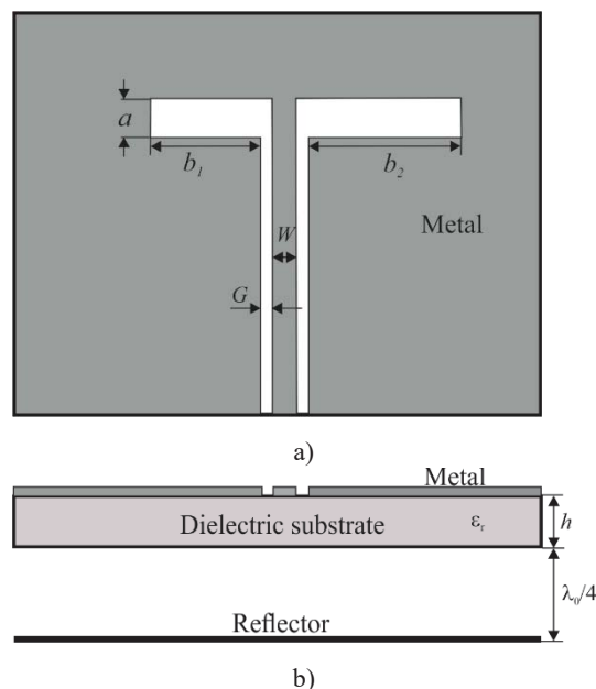
Fig. 1. CPW-fed asymmetrical rectangular slot: a) top view b) side view.
