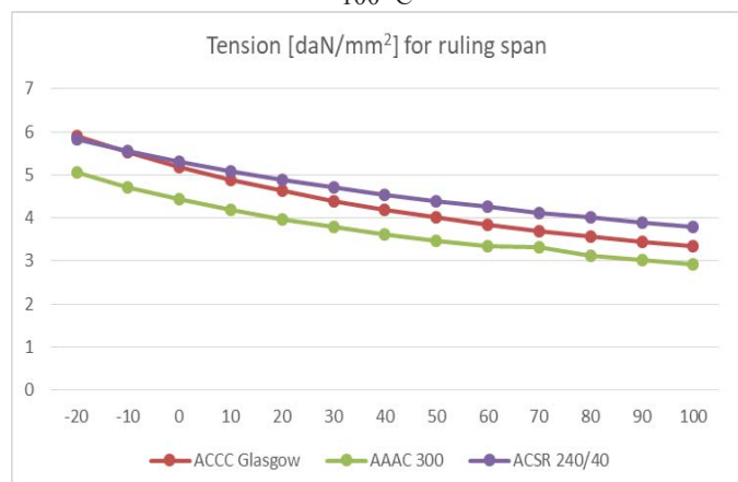
Fig. 5. Tensions for ruling span for full range of temperatures -20 °C to 100 °C
